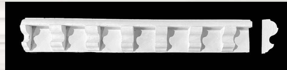
AC036 Modillion Size: 1625 x 65 x 25
