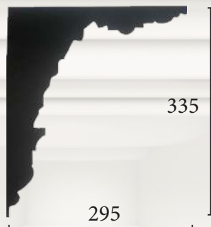
CR010 Egg & Dart With Floral Moulding.
