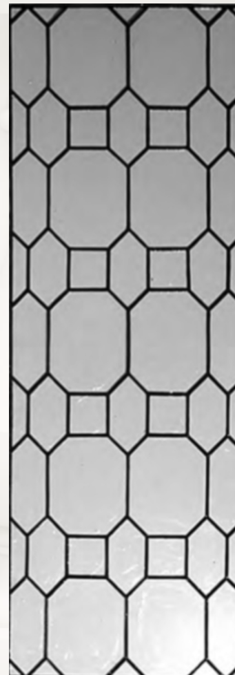
WG022 14th Century Sheet Size: 1922 x 680 x 10
